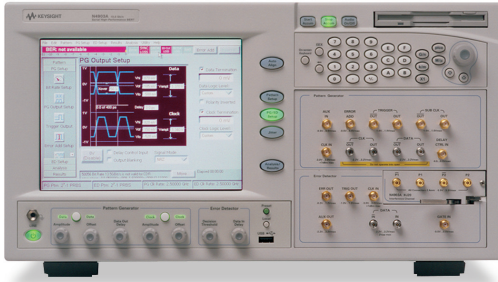
Pair a W2641B TPA with an Keysight N4903B J-BERT or E4887A ParBERT (81250) for DisplayPort sink validation.
