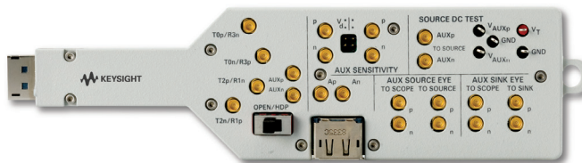
The W2641B DisplayPort test point access adapter
