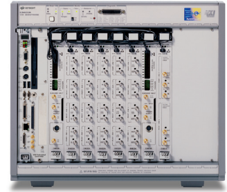
Pair a W2641B TPA with an Keysight N4903B J-BERT or E4887A ParBERT (81250) for DisplayPort sink validation.
